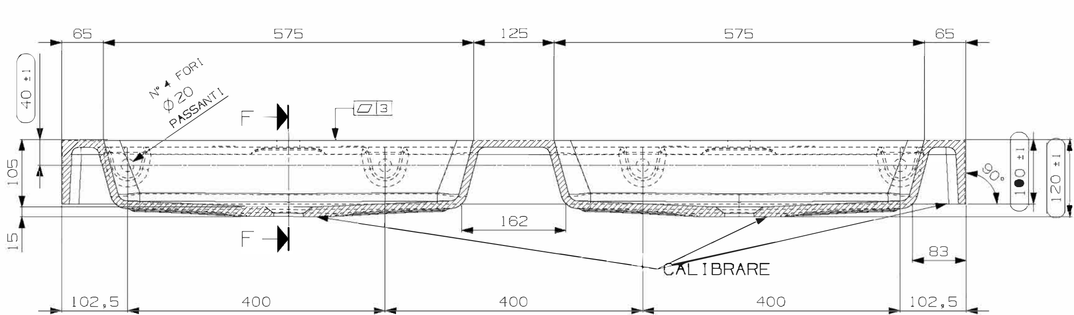
SECTION E-E SCALE 35:200
