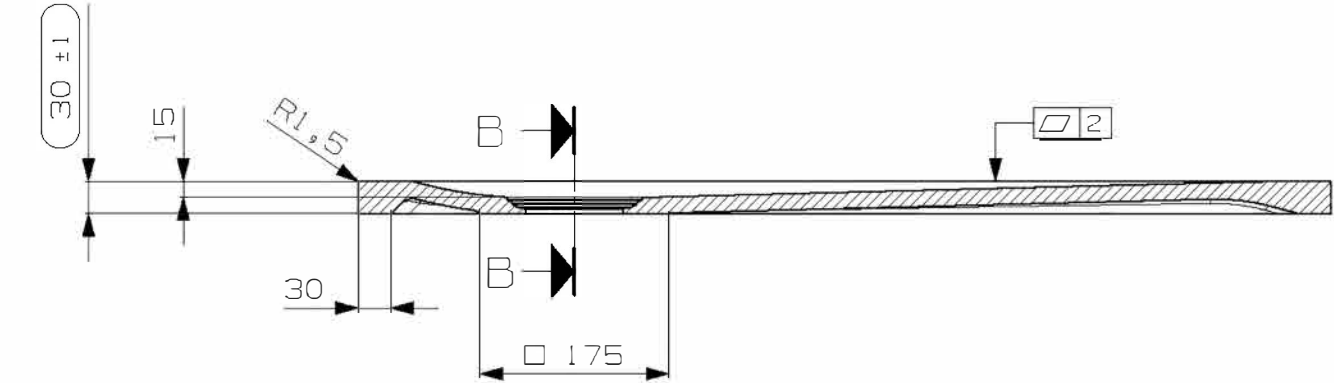
SECTION A-A SCALE 0.143:1.0
