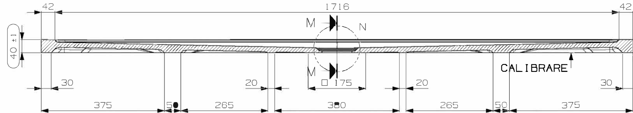
aqualorte 42 716 42 2 SPIGOLATURA 1X1 SECTION M-M SCALE 0.143:1.0
