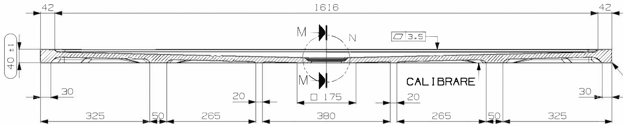
SECTION L-L SCALE 0.143:1.0
