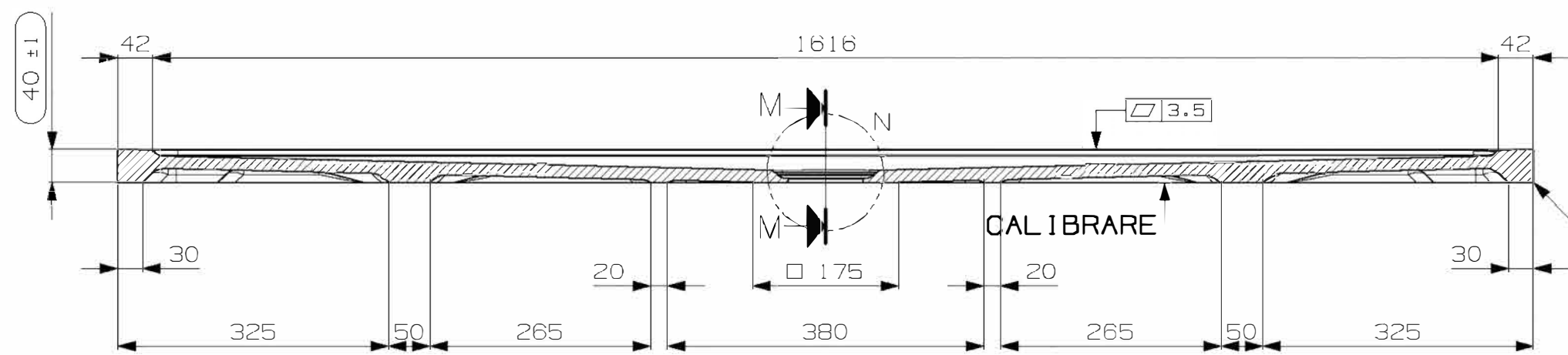
SECTION L-L SCALE 0.143:1.0
