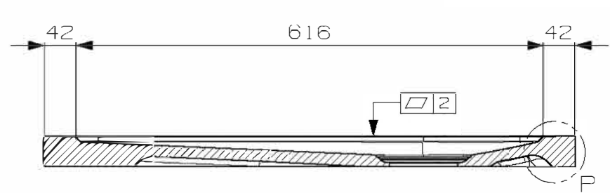
SECTION M-M SCALE 0.143:1.0
