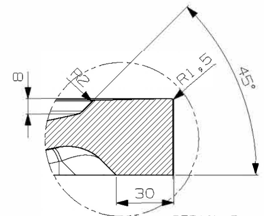
DETAIL P SCALE 1:2
