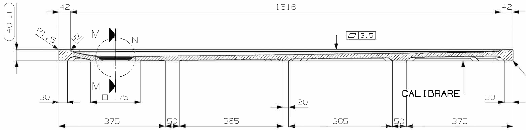
SECTION L-L SCALE 0.143:1.0
