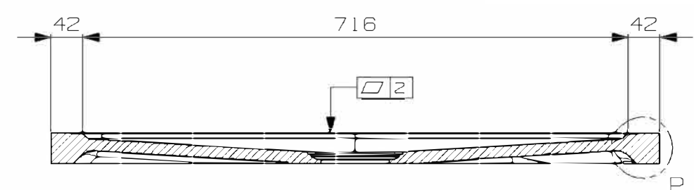
SECTION M-M SCALE 0.143:1.0
