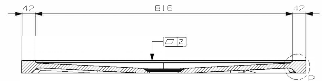
SECTION M-M SCALE 0.143:1.0
