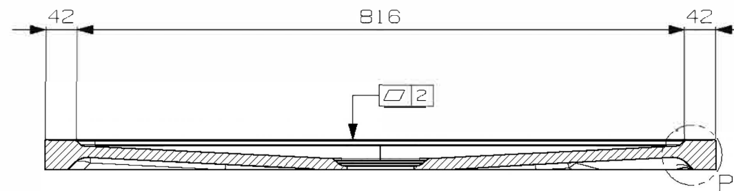
SECTION M-M SCALE 0.143:1.0
