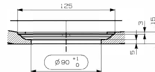
DETAIL B SCALE 1:2
